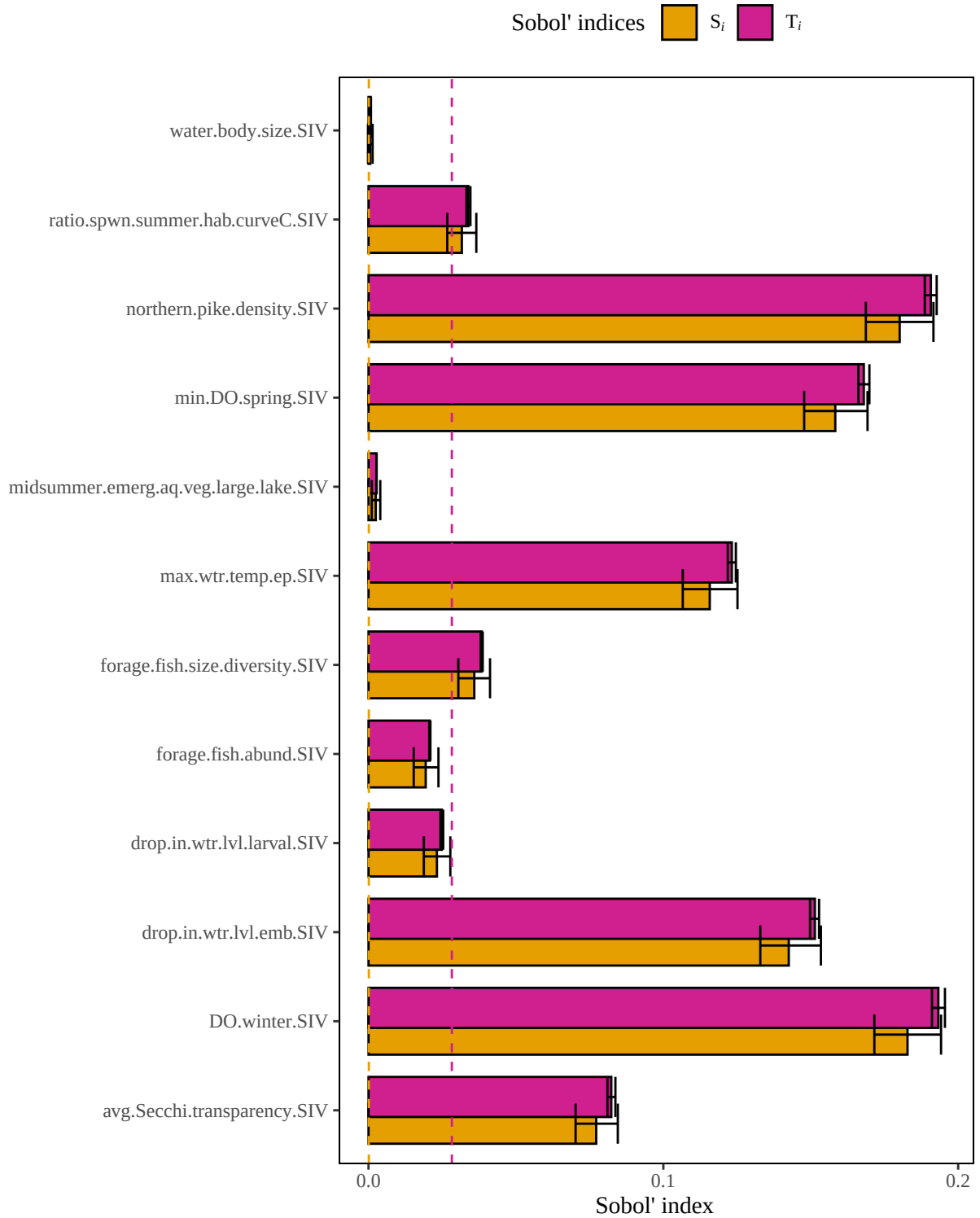
Figure 5. Results of a sensitivity analysis for the muskellungeLargeLakeSpwnVegCurveC model based on a geometric mean structure. Dashed lines represent baseline numerical approximation error for S_i and T_i ( i.e. , dummy variables).
