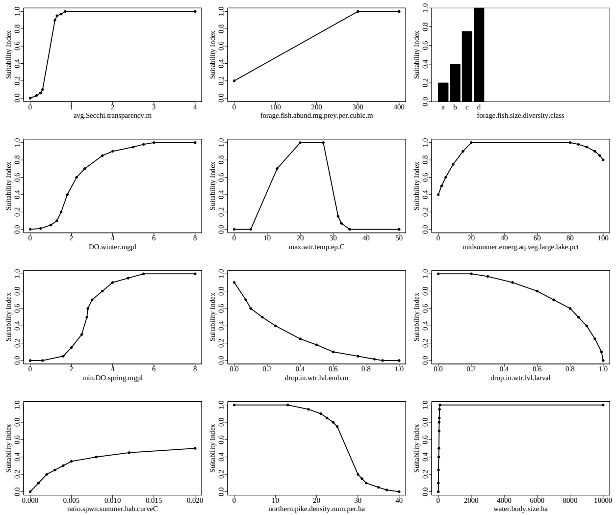
Figure 1. Suitability index graphs for variables included in the muskellungeLargeLakeSpwnVegCurveC model in ecoest.
